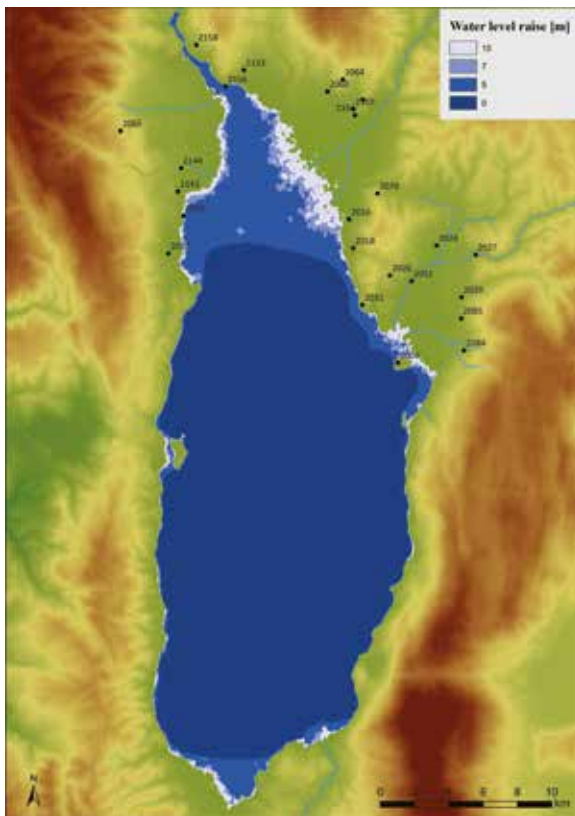
Pl. 1/2: Model of water level raising in the Ohrid Lake (map by M. Jančovič).
